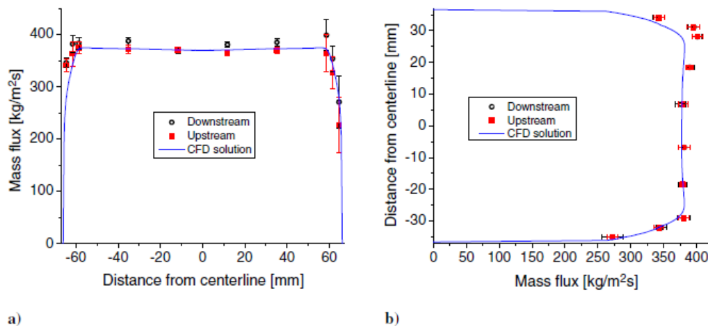
Figure 2.7. Spatially resolved mass flux at Mach 7 condition plotted from a) left to right of channel (facing downstream) in vertical planes and b) top to bottom of channel in horizontal planes. Reproduced with permission from the authors.
